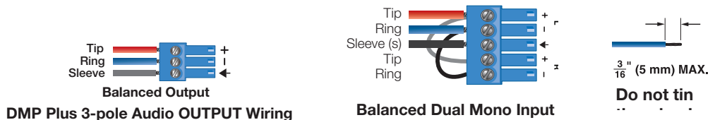
Figure 3. Captive Screw Audio Cable Wiring
