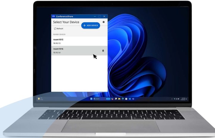
Starting ConferenceShare
